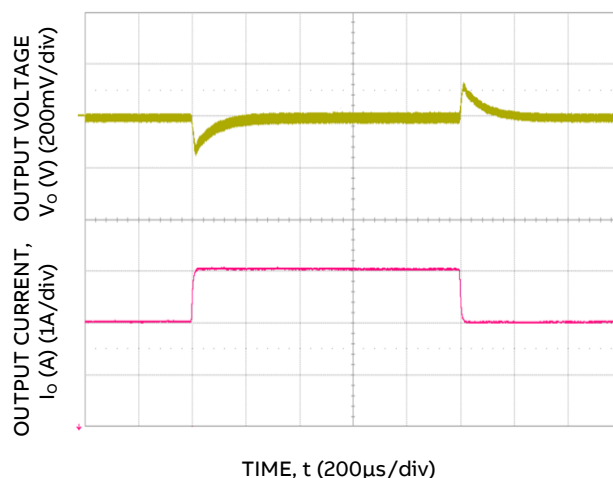
Figure 4. Transient Response to 0.1A/μs Dynamic load Change from 50% to 75% to 50% of full load, V_{in}=24V , C_o > 100μF
