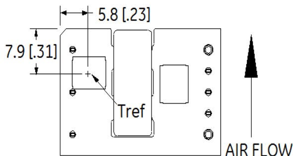
Figure 16. T_{ref} Temperature Measurement Location.
