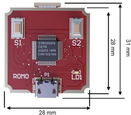
ROMO-E Electronic Driver PCB
