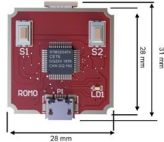
LROM Electronic Driver PCB
