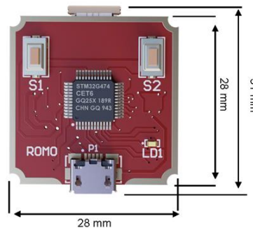
LRMO-E Electronic Driver PCB
