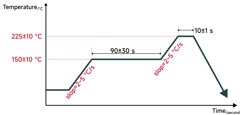
Figure 20: Soldering Temperature Profile for KTH7801 Series
