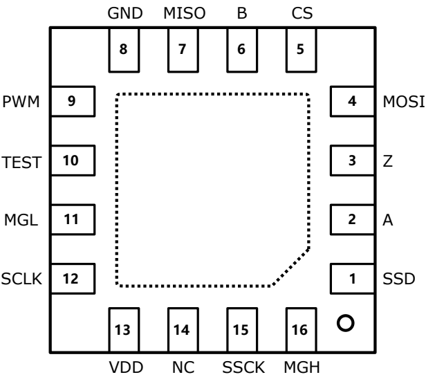
Figure 3: QFN-16L 3mmx3mm
