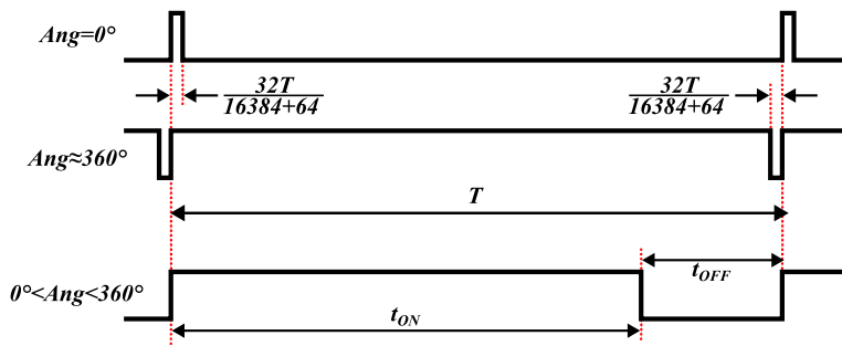
Figure 14: PWM Timing
