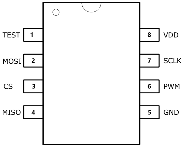
Figure 4: SOP-8 4.9mmx6mm
