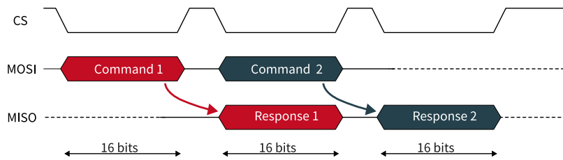
Figure 9: SPI Command-Response Overlapped Structure
