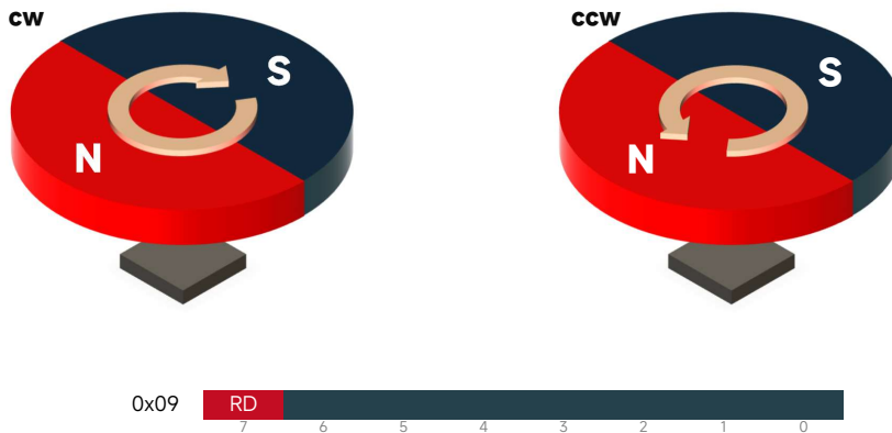
Figure 15: Rotation Direction
